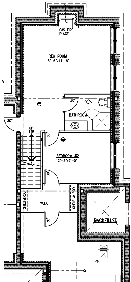
Basement Bungalow
