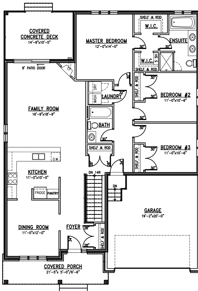
MainFloor
