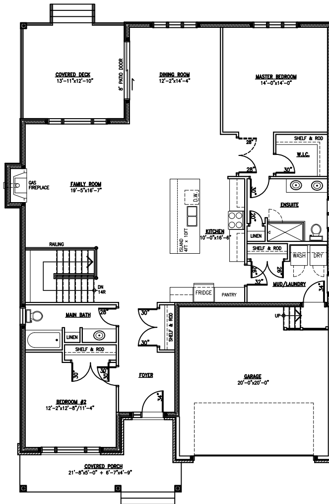
MainFloor
