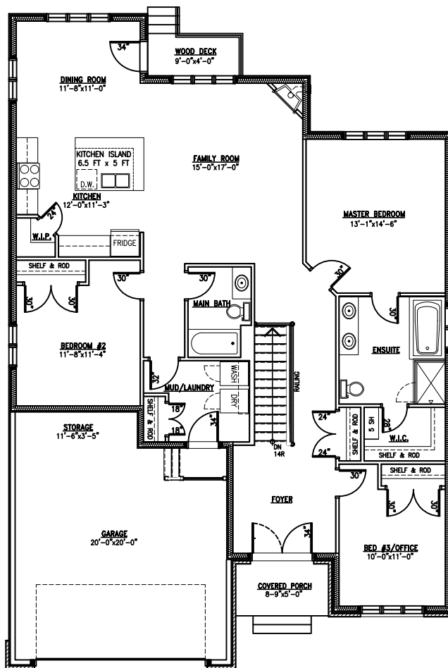
MainFloor
