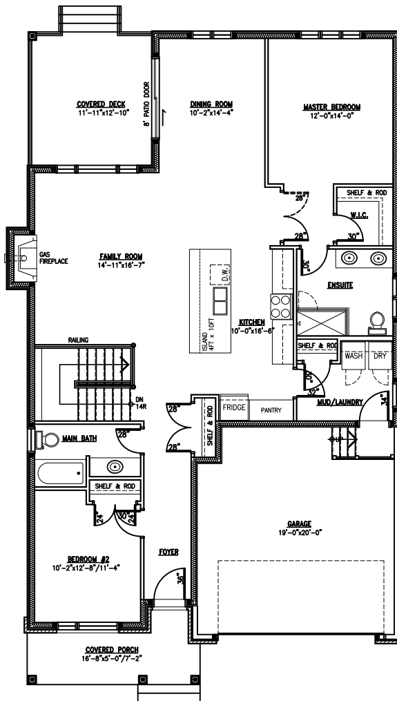
MainFloor
