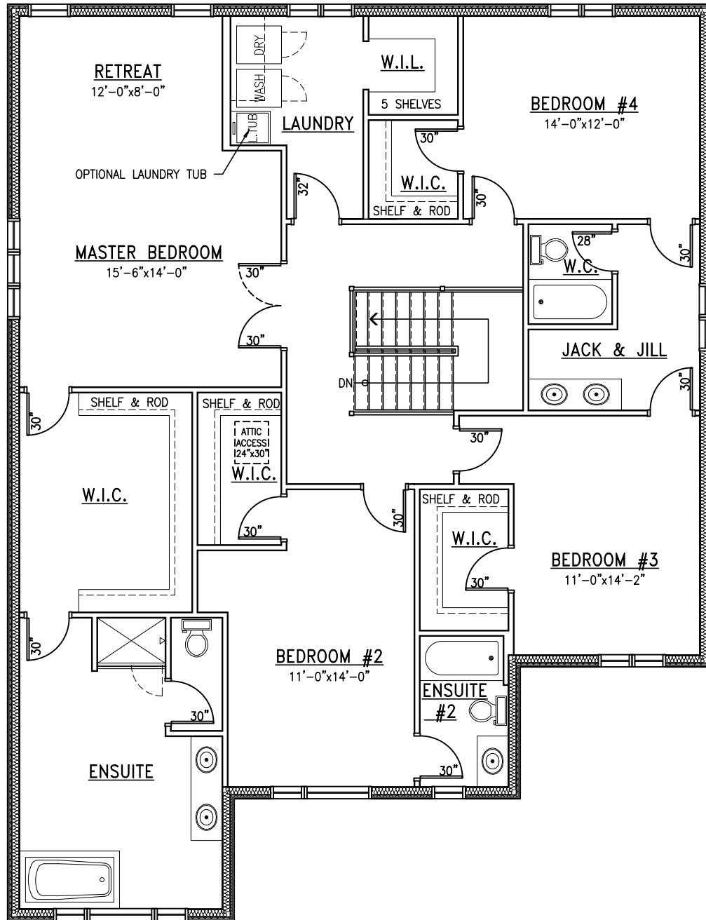
Second Floor
