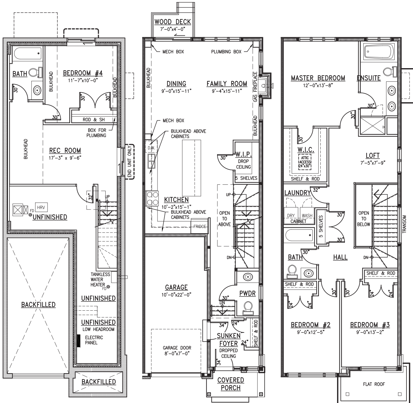
Basement
