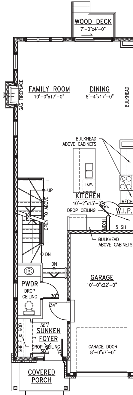
Ground Floor
