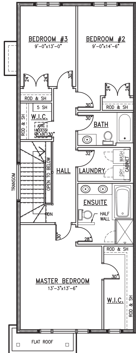
Second Floor
