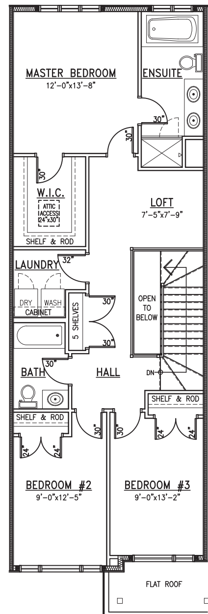
Second Floor
