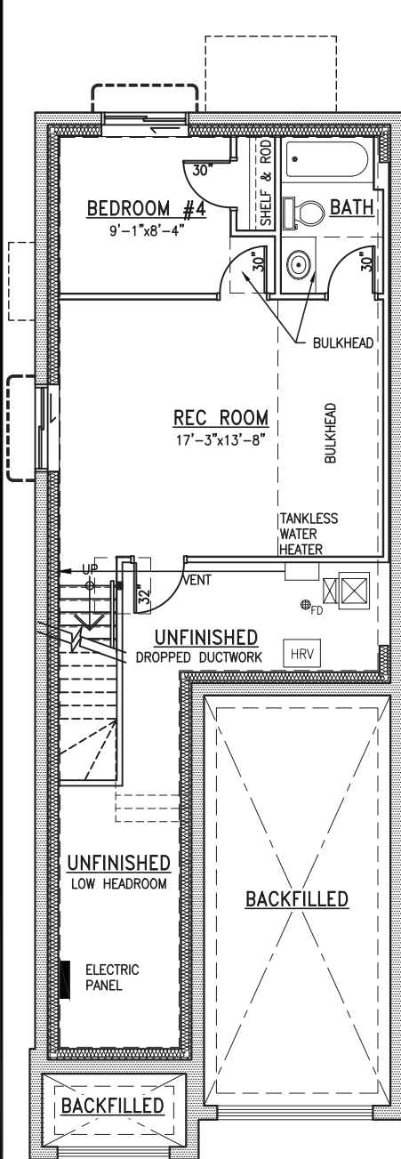
Basement
