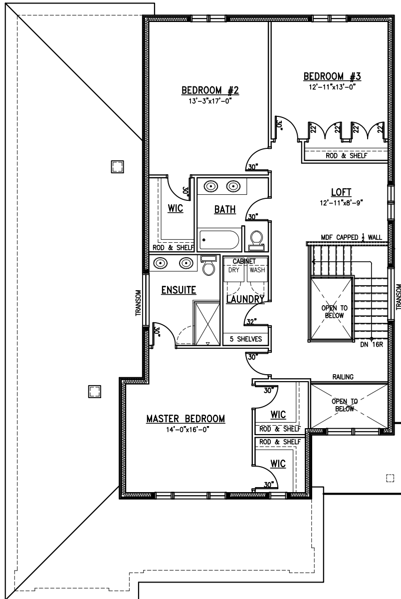
Second Floor 1,465 SQ FT
